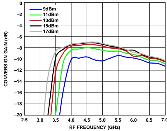
Figure 54. Conversion Gain vs. RF Frequency at Various LO Powers
