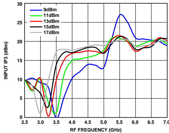
Figure 55. Input IP3 vs. RF Frequency at Various LO Powers
