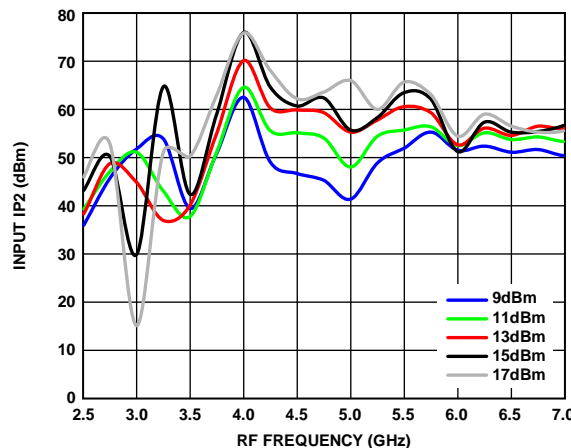
Figure 56. Input IP2 vs. RF Frequency at Various LO Powers
