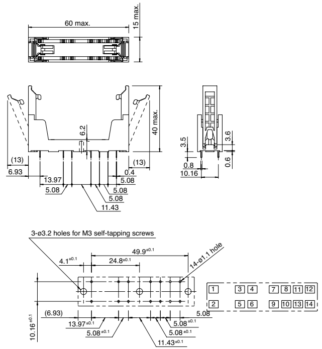
SF1V-6-07L (6-pole)
