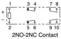
RF1V (4-pole)
