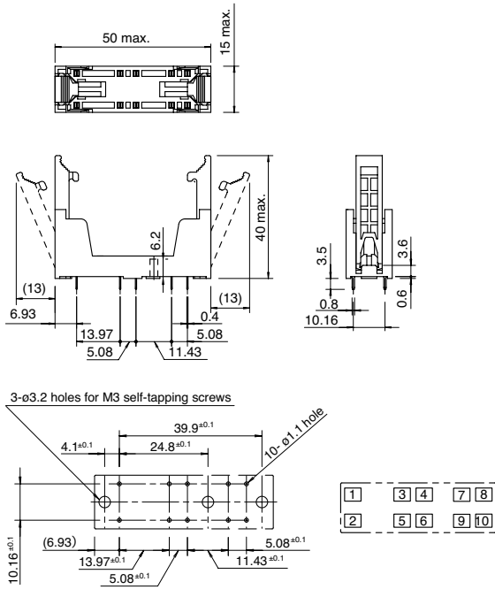
SF1V-4-07L (4-pole)
