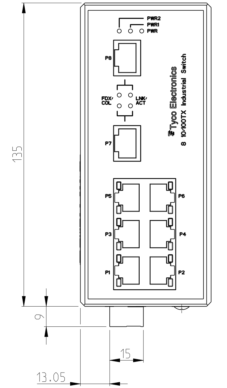
1987030-1 AS SHOWN
