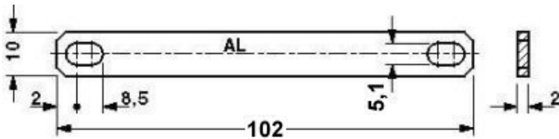
Dimensioned drawing
